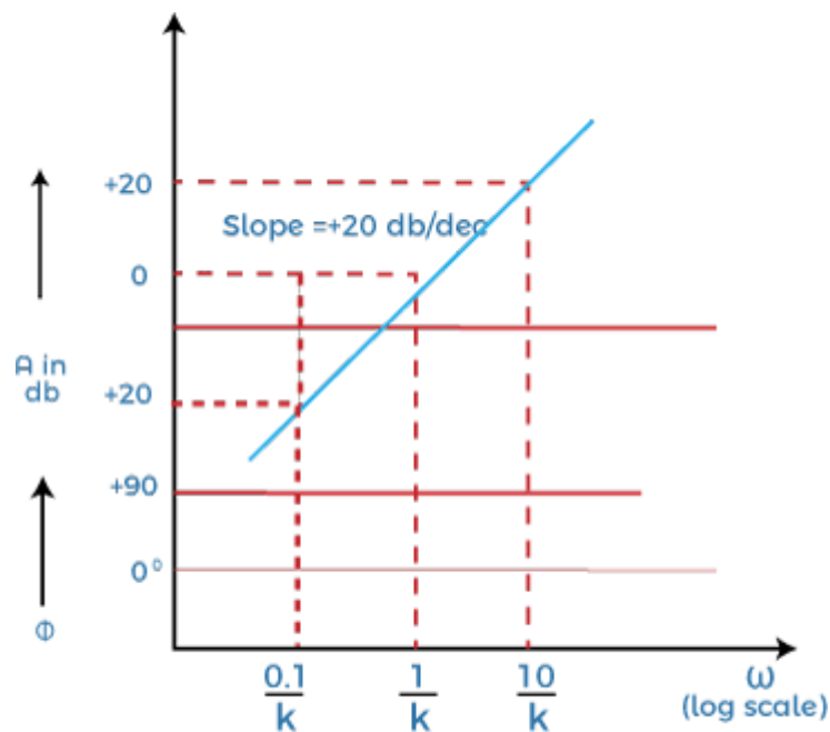
Bode plot of derivative factor, k \times j\omega
