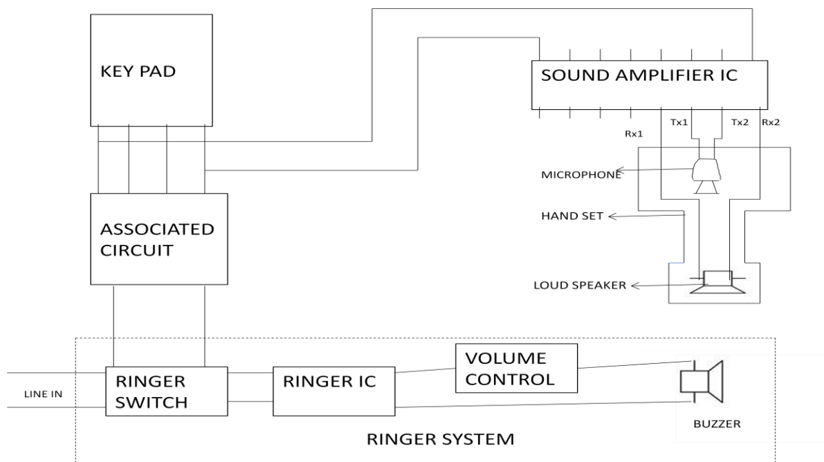
Fig. 4.1 Telephone Base Unit
