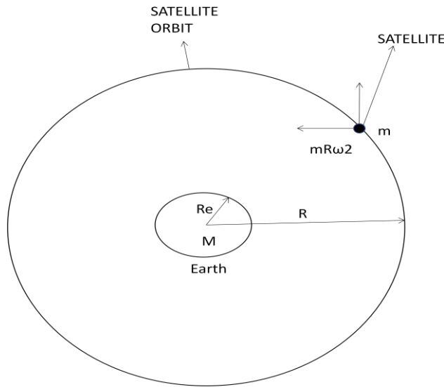
Fig. 2.1 Satellite Orbit
