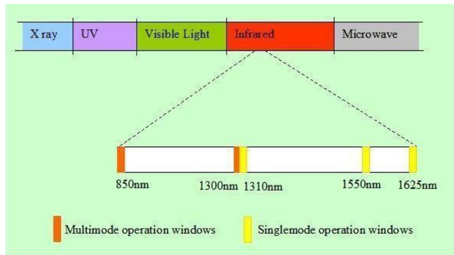
Fig. 3.2 Optical Spectrum
