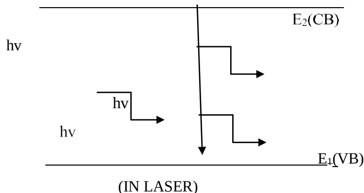
Fig. 3.8 Electron emission
