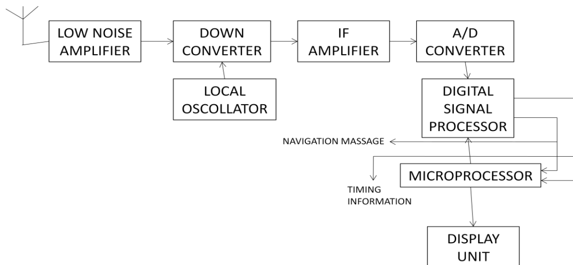
Fig. 2.8 GPS Receiver
