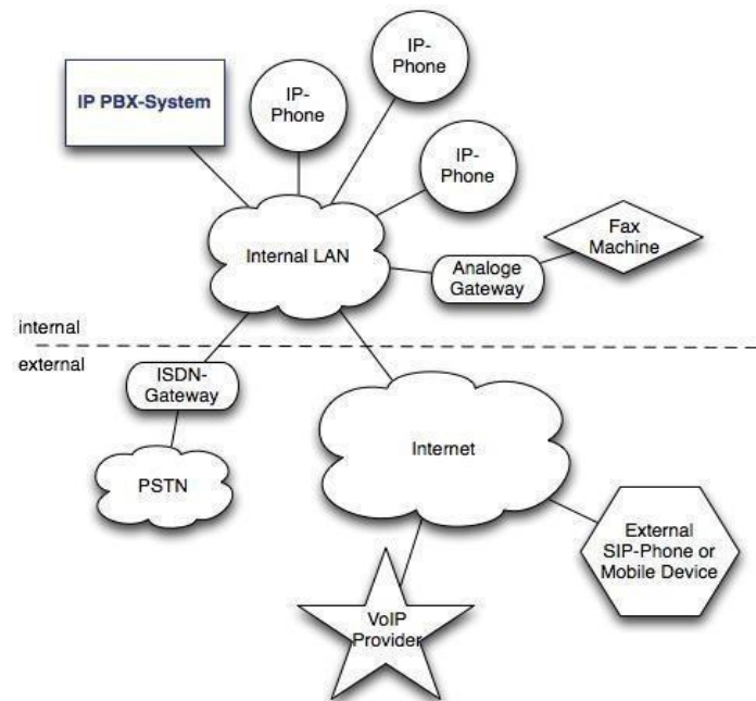
Fig. 4.3 PBX System
