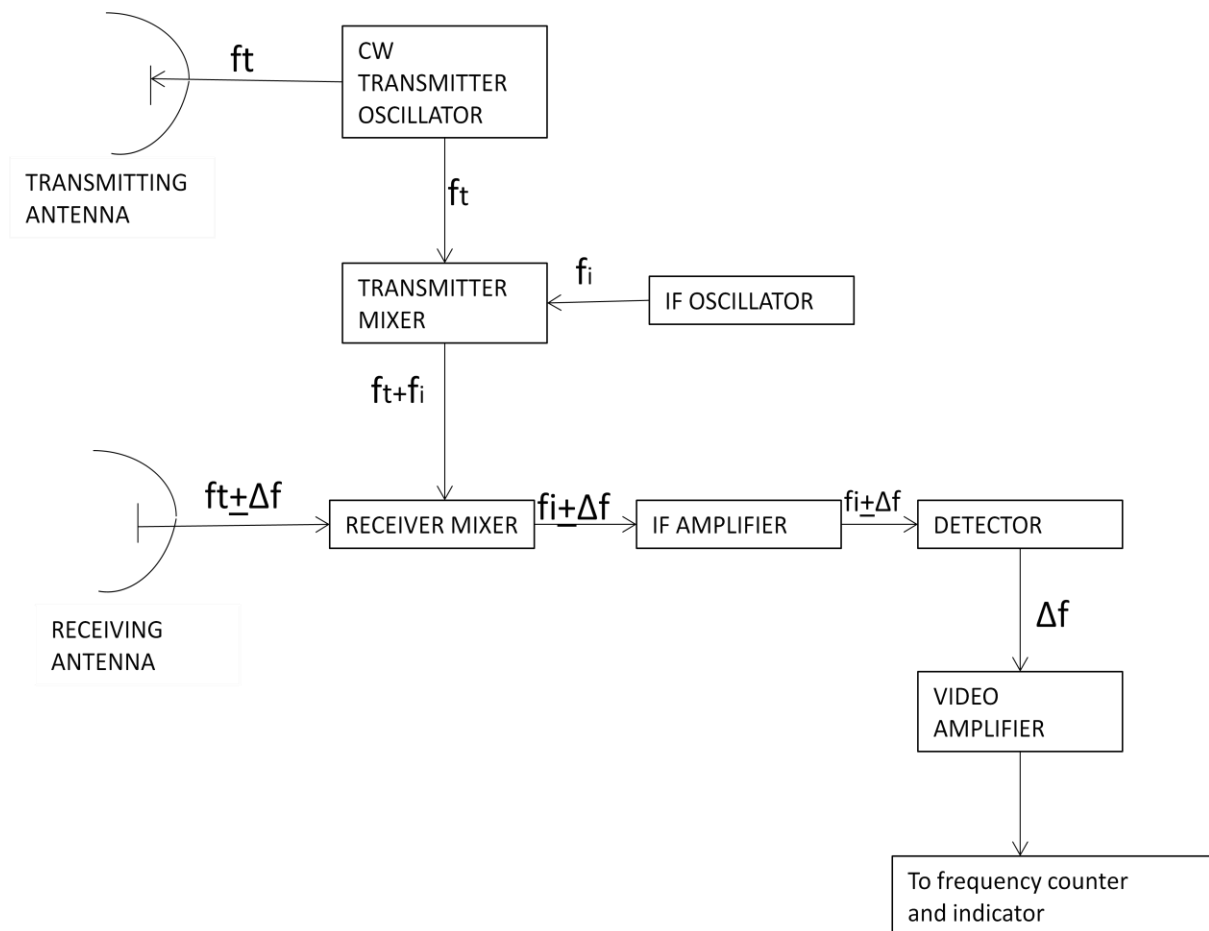
Fig. 1.3 CW RADAR Block Diagram
