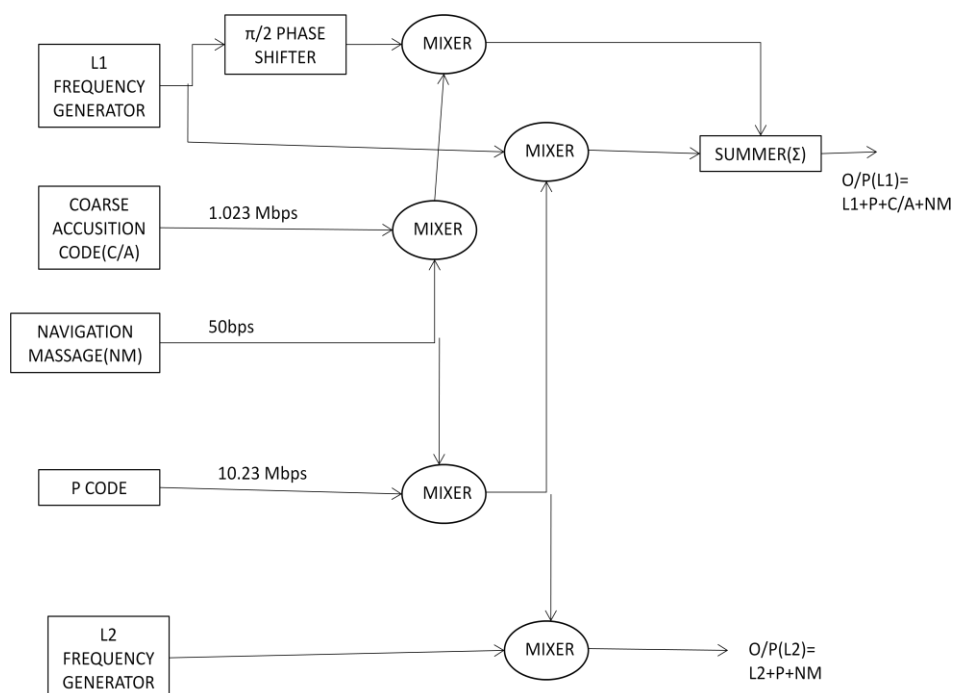
Fig. 2.7 GPS Transmitter
