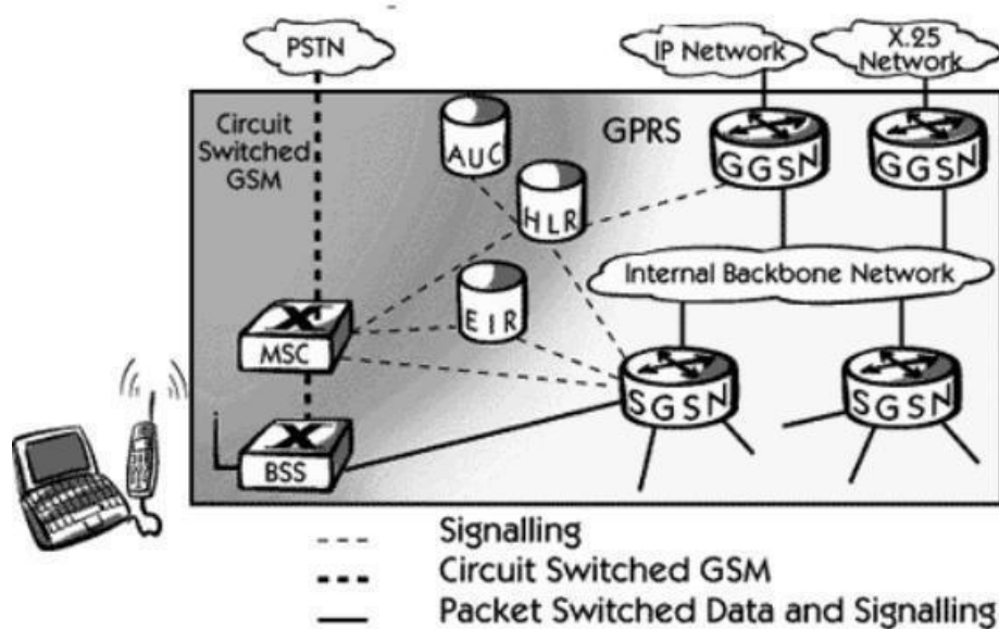
Fig. 6.8 GPS Architecture
