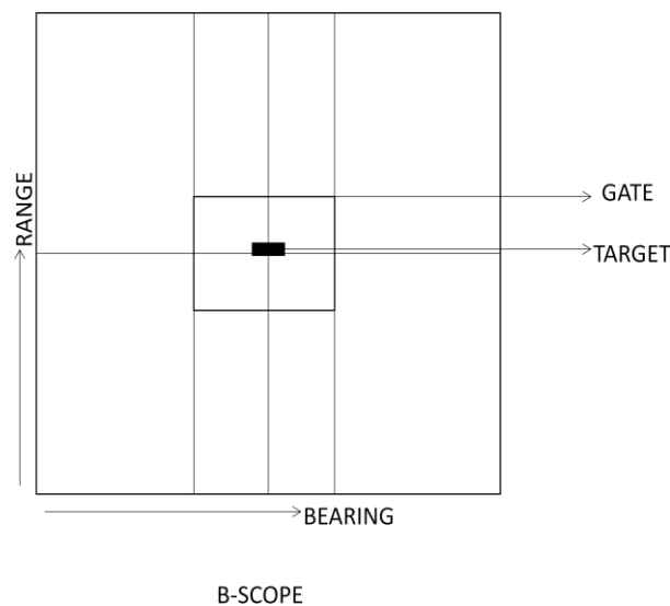
Fig. 1.7 B- Scope Indicator
