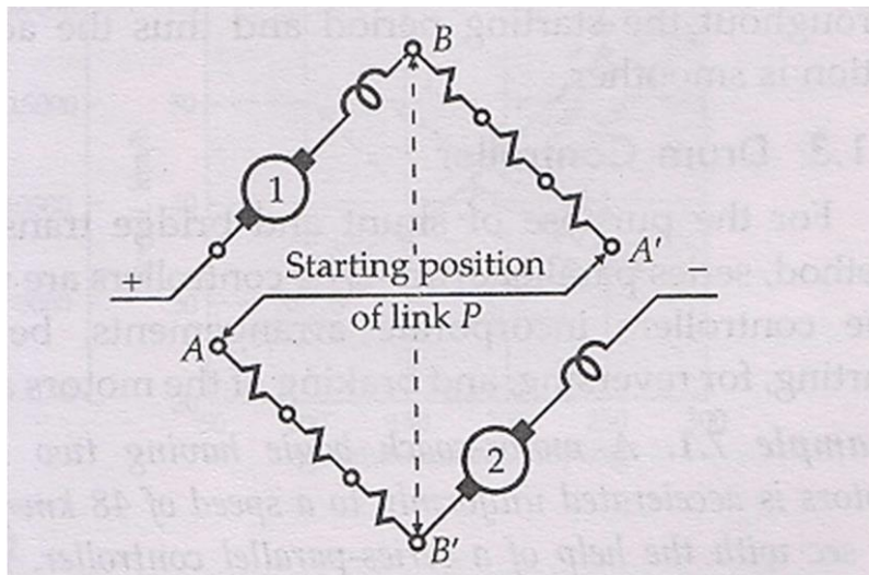
Fig.9. Series position.
