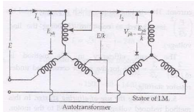
Fig.4 Autotransformer starting principle
