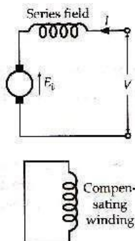
Fig.4. Circuit diagram for an inductively compensating series motor
