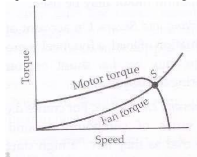
Fig.24 Fan load and induction motor torque speed curves
