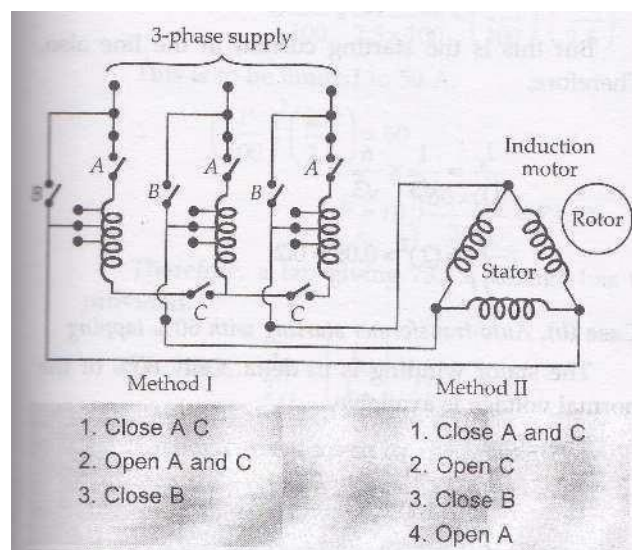
Fig. 3. Starting of SQIM by Autotransformer starter
