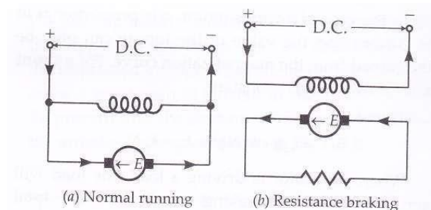
Fig..22 Rheostatic braking of shunt motor
