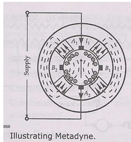
Fig.12 Illustrating Metadyne
