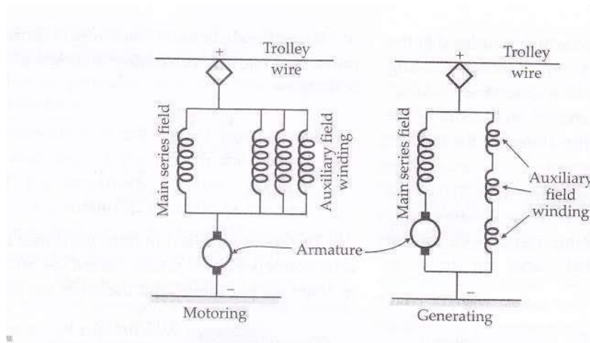
Fig. 20 Regenerative braking
