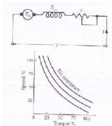
Fig.13 Speed control of series motor with series resistance in armature
