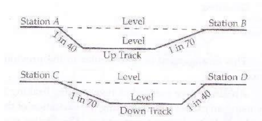
Fig.18 Track Grading
