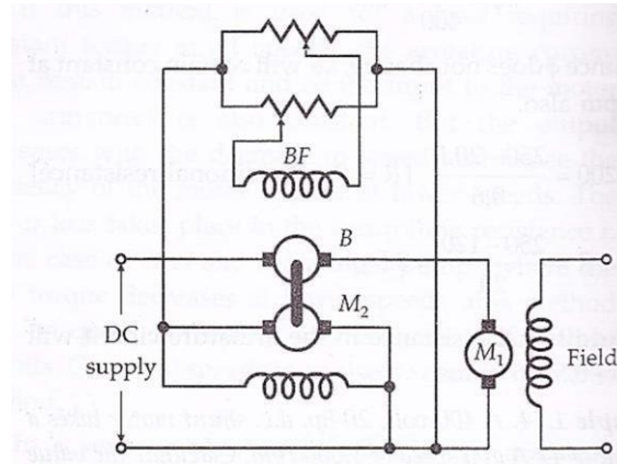
Fig.16 Booster control
