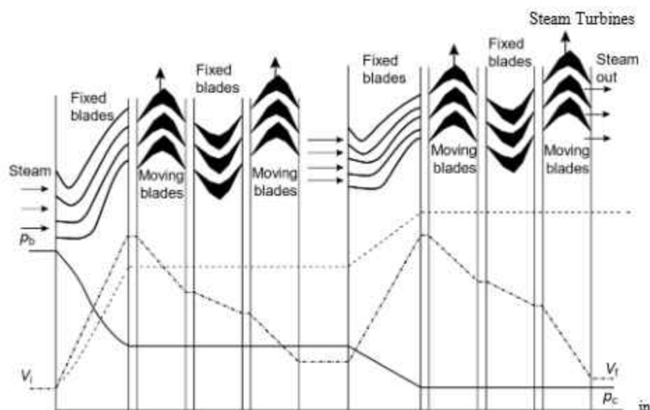
Fig. 10.7 Pressure-Velocity Compounding
