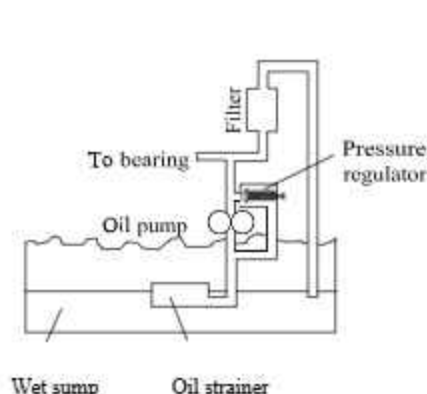
Fig. 13.20 Wet Sump Lubrication System
