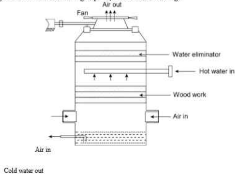
Fig. 11.16 Induced Draught Cooling Tower
