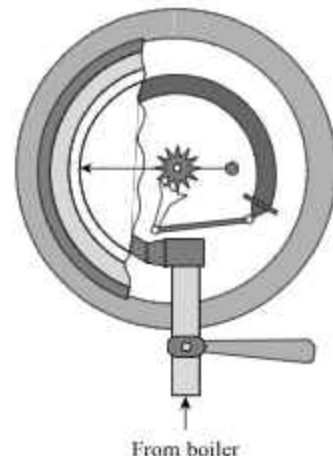
Fig. 5.33 Pressure Gauge
