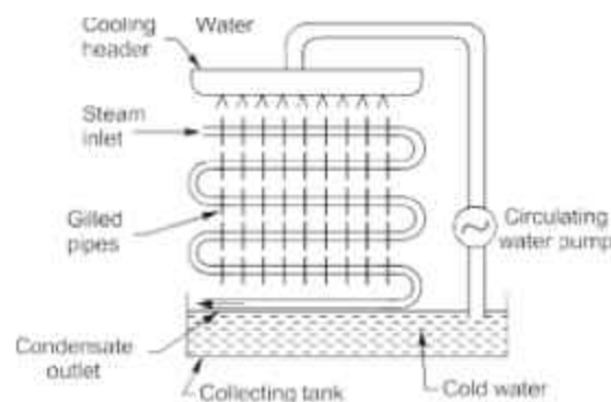
Fig. 1.26. Evaporative Condenser
