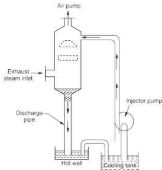
Fig. 1.21. High Level Jet Condensers
