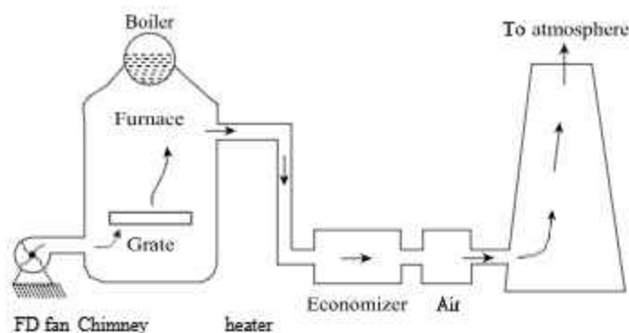
Fig. 7.2 Forced Draught
