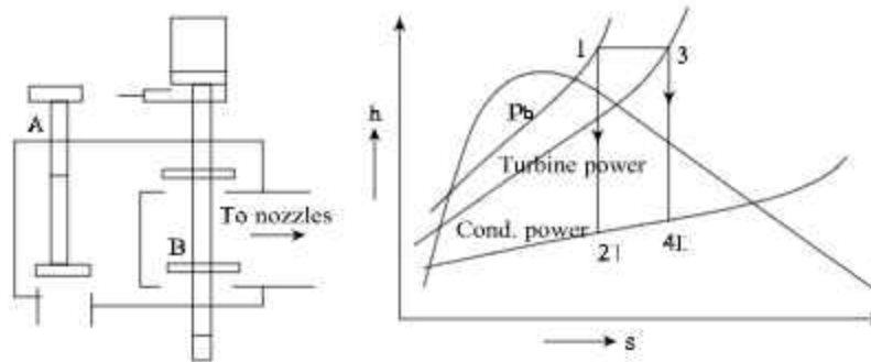
Fig. 10.18 Throttle Governor
