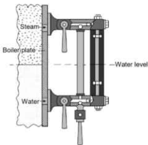
Fig. 5.32 Water-Level Indicator
