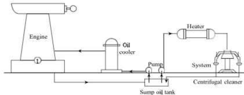
Fig. 13.27 Continuous Centrifuging System
