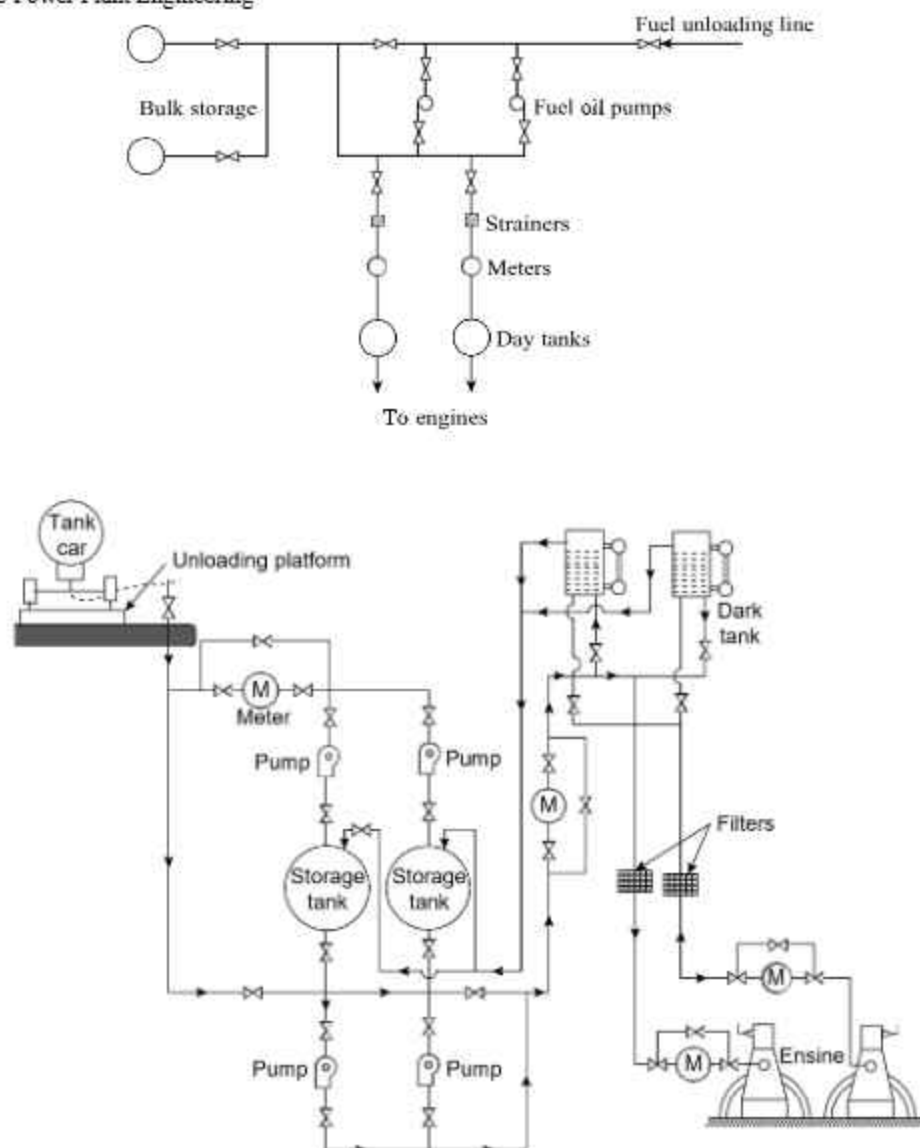
Fig. 13.8 System of Fuel Storage for a Diesel Power Plant
