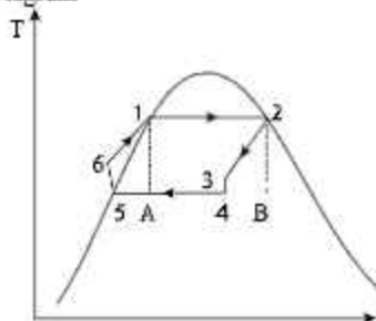
Fig. 4.19 Ideal Regenerative T-s Diagram
