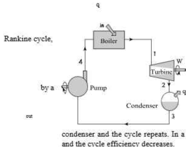
Fig. 4.5 Rankine Cycle
