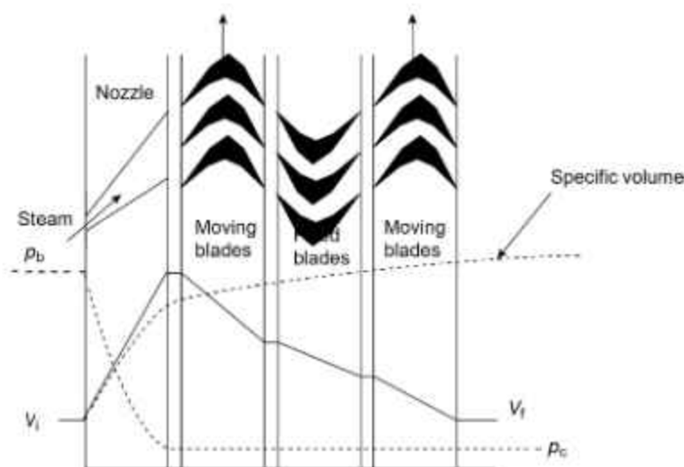
Fig. 10.5 A Simple Velocity Compounded Impulse
