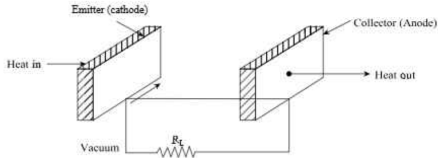
Fig. 1.11 Thermionic Converter
