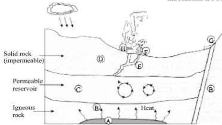
Fig. 1.8 A Typical Geothermal Field: F-fumaroles; E-fissures; H-Well; G-
