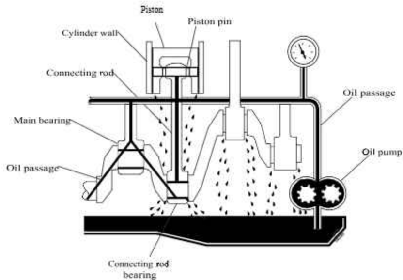
Fig. 13.24 Full Force-Feed (Pressure) Lubrication System
