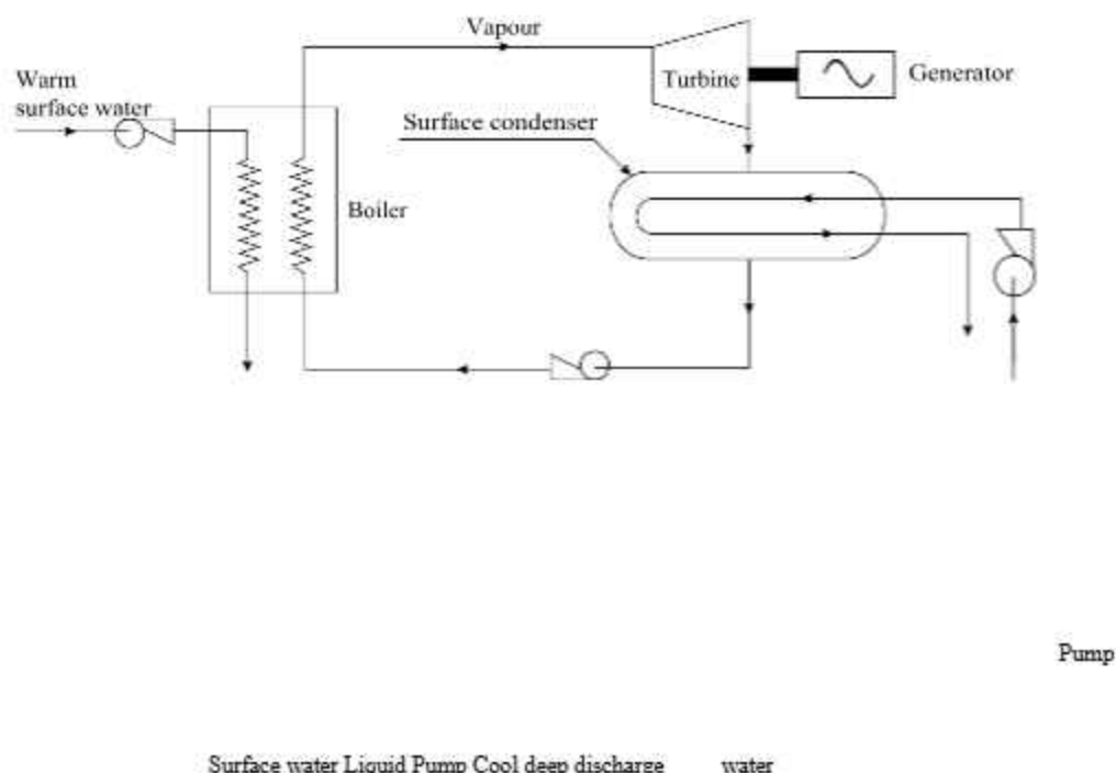
Fig. 1.5 An OTEC Plant
