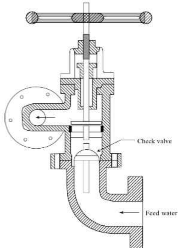
Fig. 5.35 Feed Check Valve
