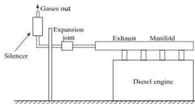
Fig. 13.29 Engine Exhaust System
