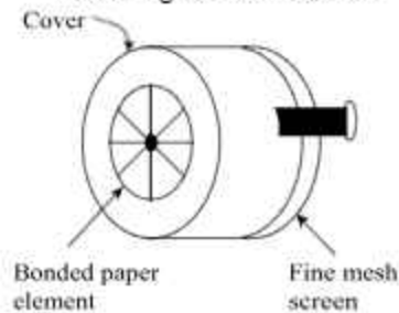
Fig. 13.26 Light Duty Air Cleaner (Dry)
