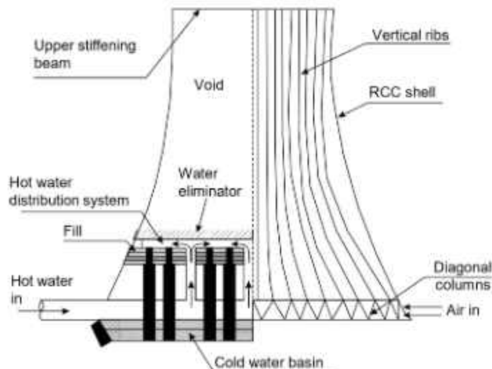
Fig. 11.10 Natural Draft Counter-Flow Cooling
