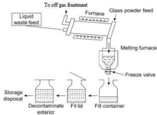
Fig. 16.37 AVM Process
