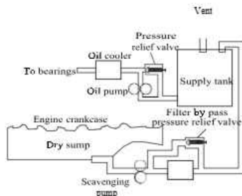
Fig. 13.21 Dry Pump Lubrication System
