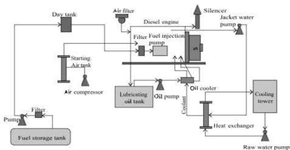
Fig. 13.6 General Layout of DG Plant
