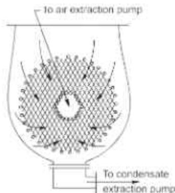
Fig. 1.25. Central Flow Surface Condensers
