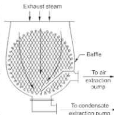
Fig. 1.24. Downflow
