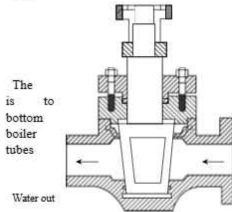
Fig. 5.36 Blow-Down Valve
