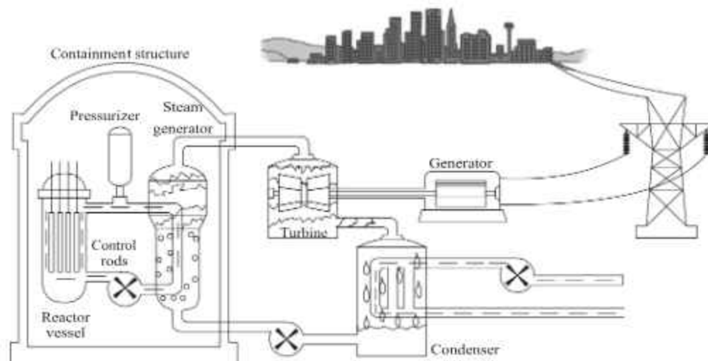
Fig. 3.8. The Pressurized Water Reactor
