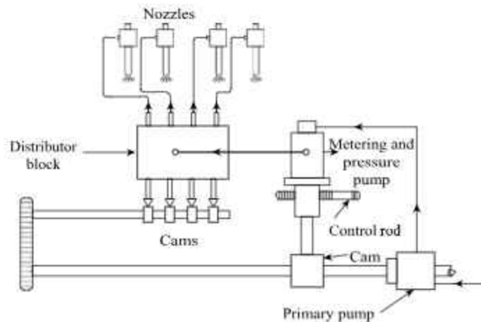
Fig. 13.12 Distributor System
