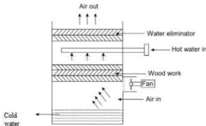
Fig. 11.15 Mechanical Draught Cooling Tower
