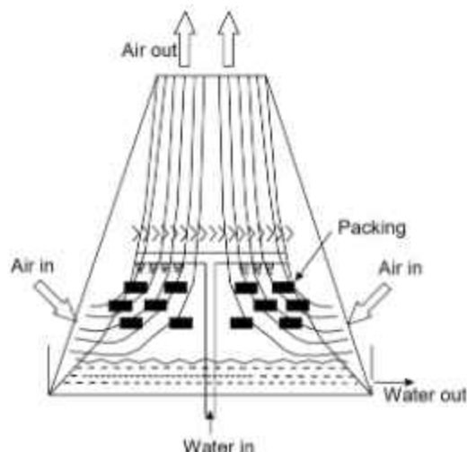
11.14 Hyperbolic Cooling Tower
