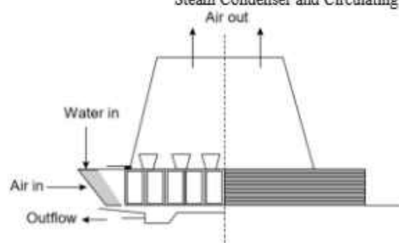
Fig. 11.17 Hybrid Cooling Tower
