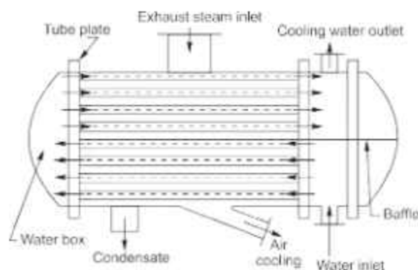
Fig. 1.23. Surface Condenser
