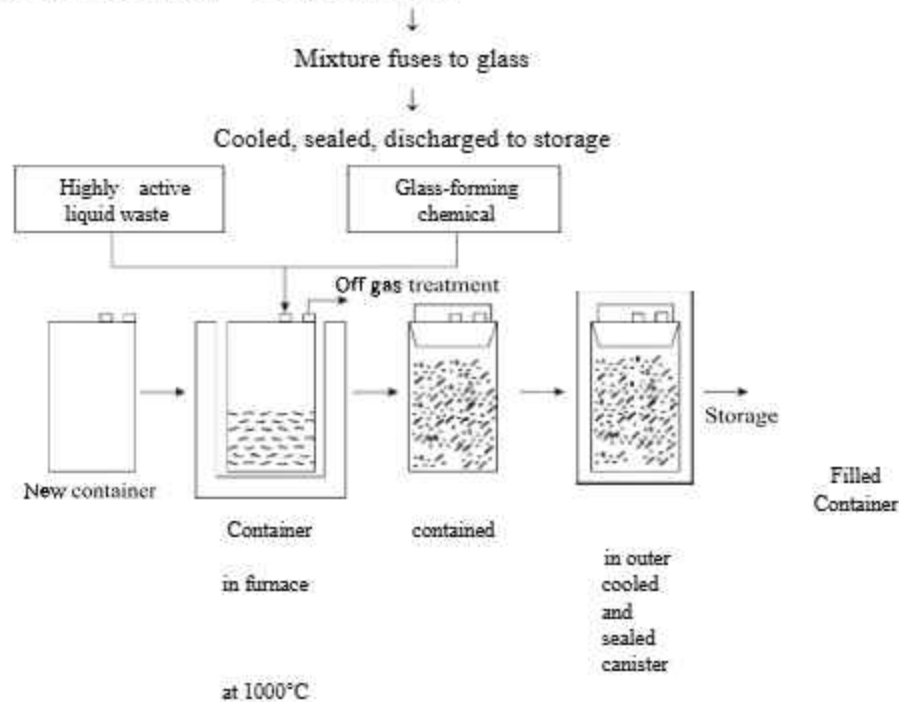
Fig. 16.36 Waste Treatment (HARVEST Process)
