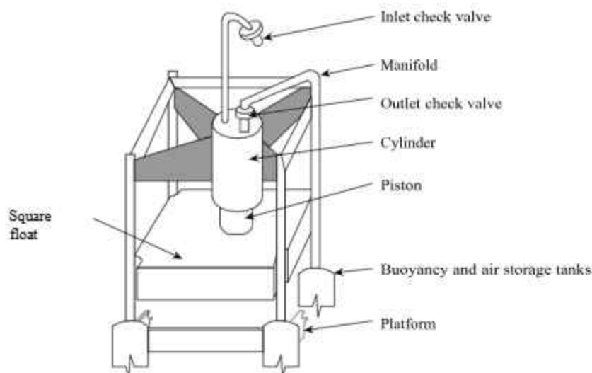
Fig. 1.7 A Typical Wave Energy Conversion System
