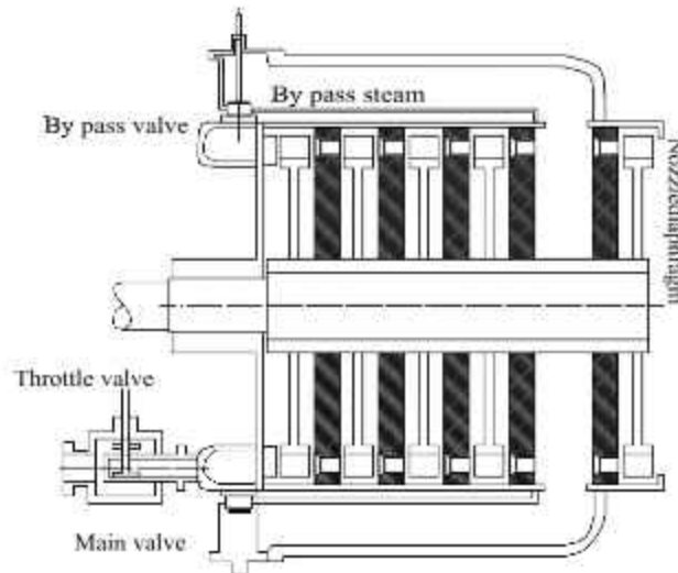
Fig. 10.20 Bypass Governing
