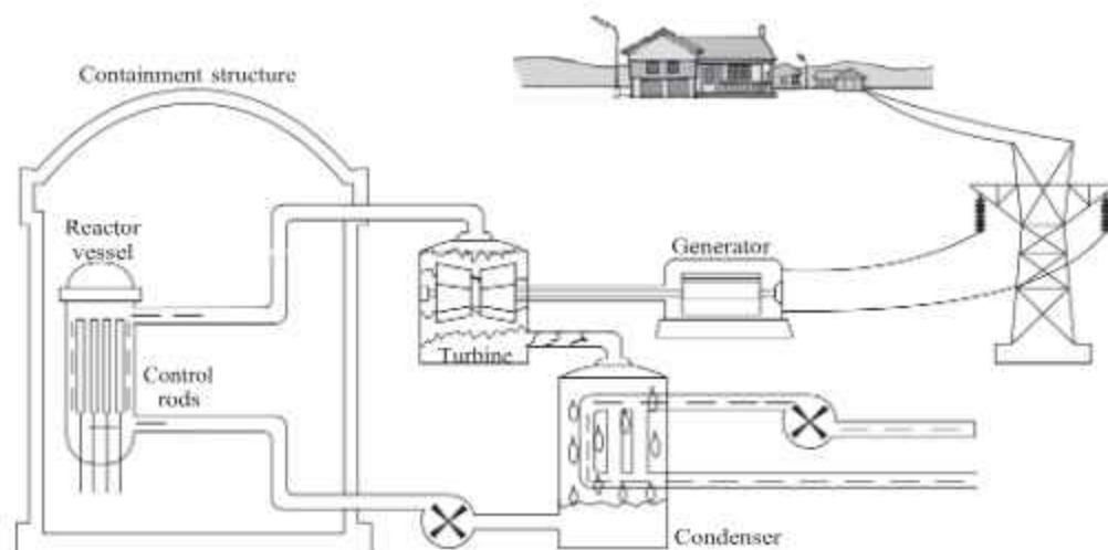
Fig. 3.9. The Boiling Water Reactor (BWR)
