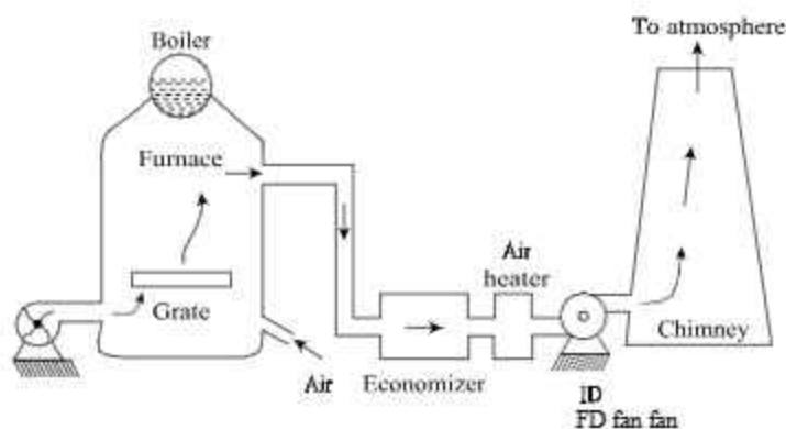
Fig. 7.3 Balanced Draught
