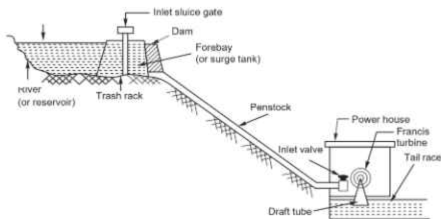
Fig. 2.1. Layout of Hydroelectric Power Plant
