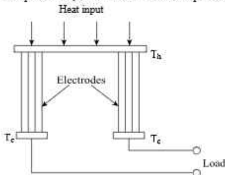
Fig. 1.12 Thermoelectric Generator
