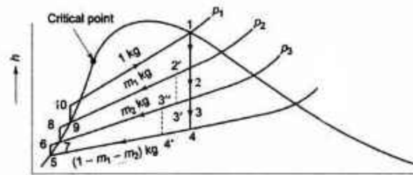
Fig. 12.21 Regenerative cycle on h - s diagram
