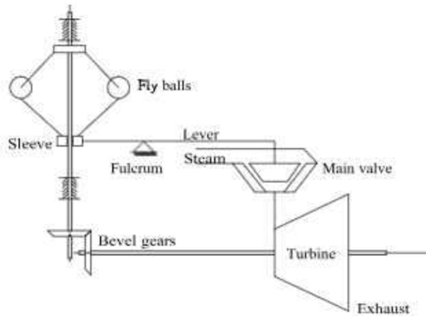
Fig. 10.17 A Centrifugal Flyball-Type Governor
