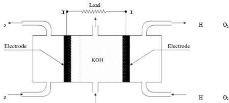
Fig. 1.9 A Hydrox Cell
