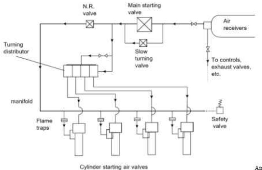
Fig. 13.14 Compressed Air System
