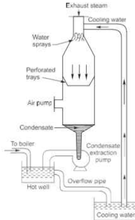
Fig. 1.19. Parallel Flow Jet Condenser
