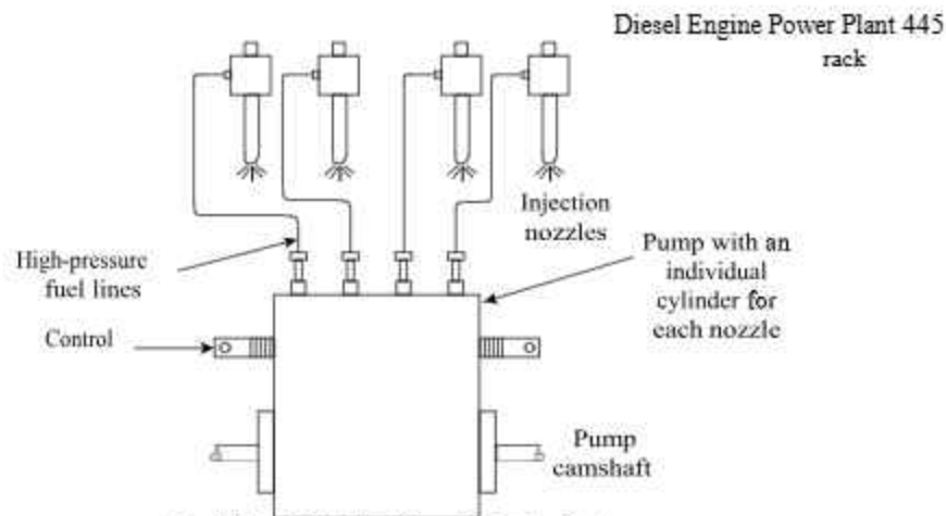
Fig. 13.11 Individual Pump Injection System
