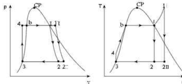
Fig. 4.6 Rankine Cycle on p - V and T - s Diagrams
