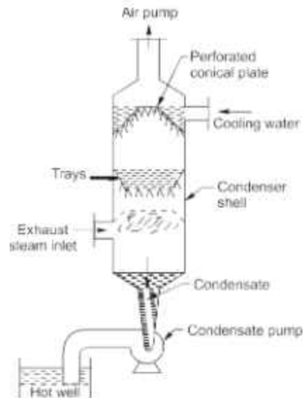
Fig. 1.20. Counter Flow Jet Condenser
