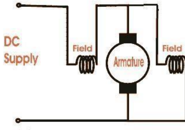
Short Shunt DC Motor
