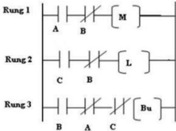
Example of Ladder Logic Program
