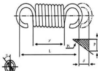
Tension
