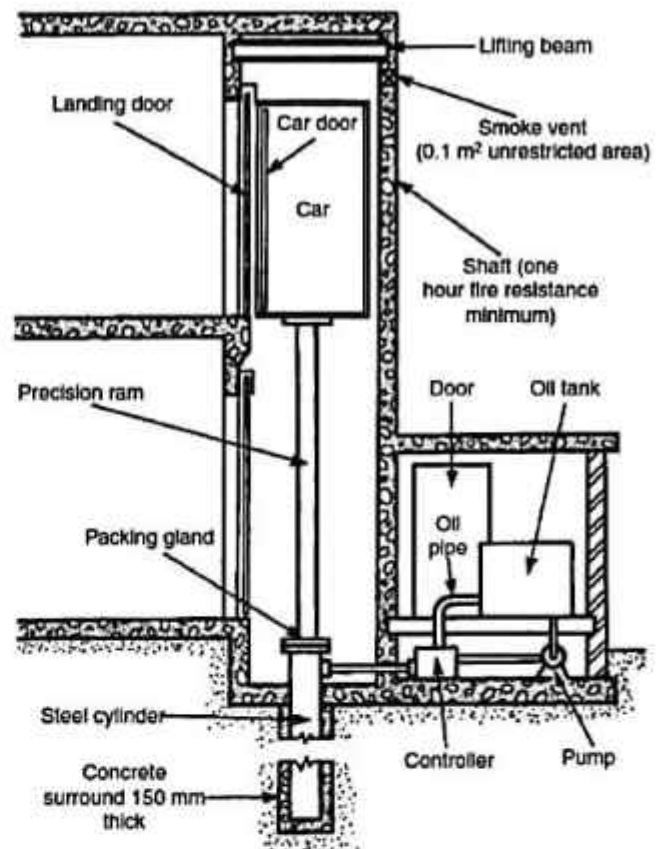
Vertical section
