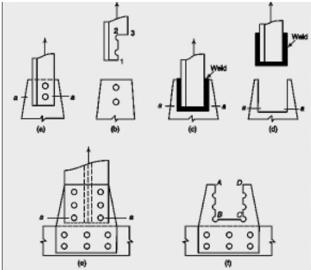
Figure 9.6 Examples Of Block Shear Failures
