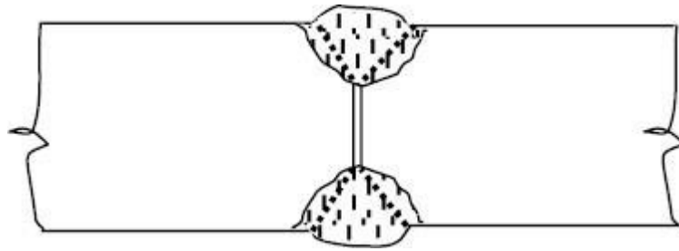
Figure 8.3 Partial penetration weld Design
