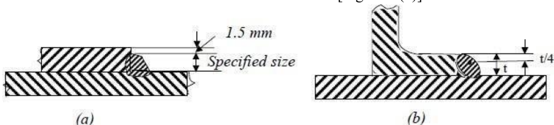
Figure 8.11 (a) fillet welds on square edge of plate, (b) fillet welds on round toe of rolled section
