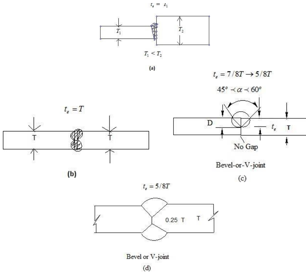
Figure 8.5 Effective throat dimensions for groove welds
