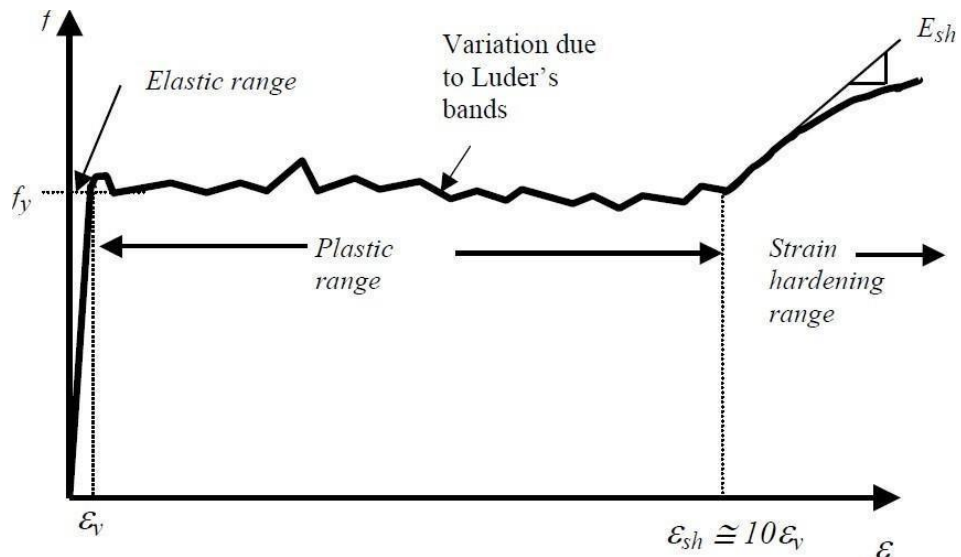
Figure 1.2 Stress-strain curve for sharp yielding structural steels
