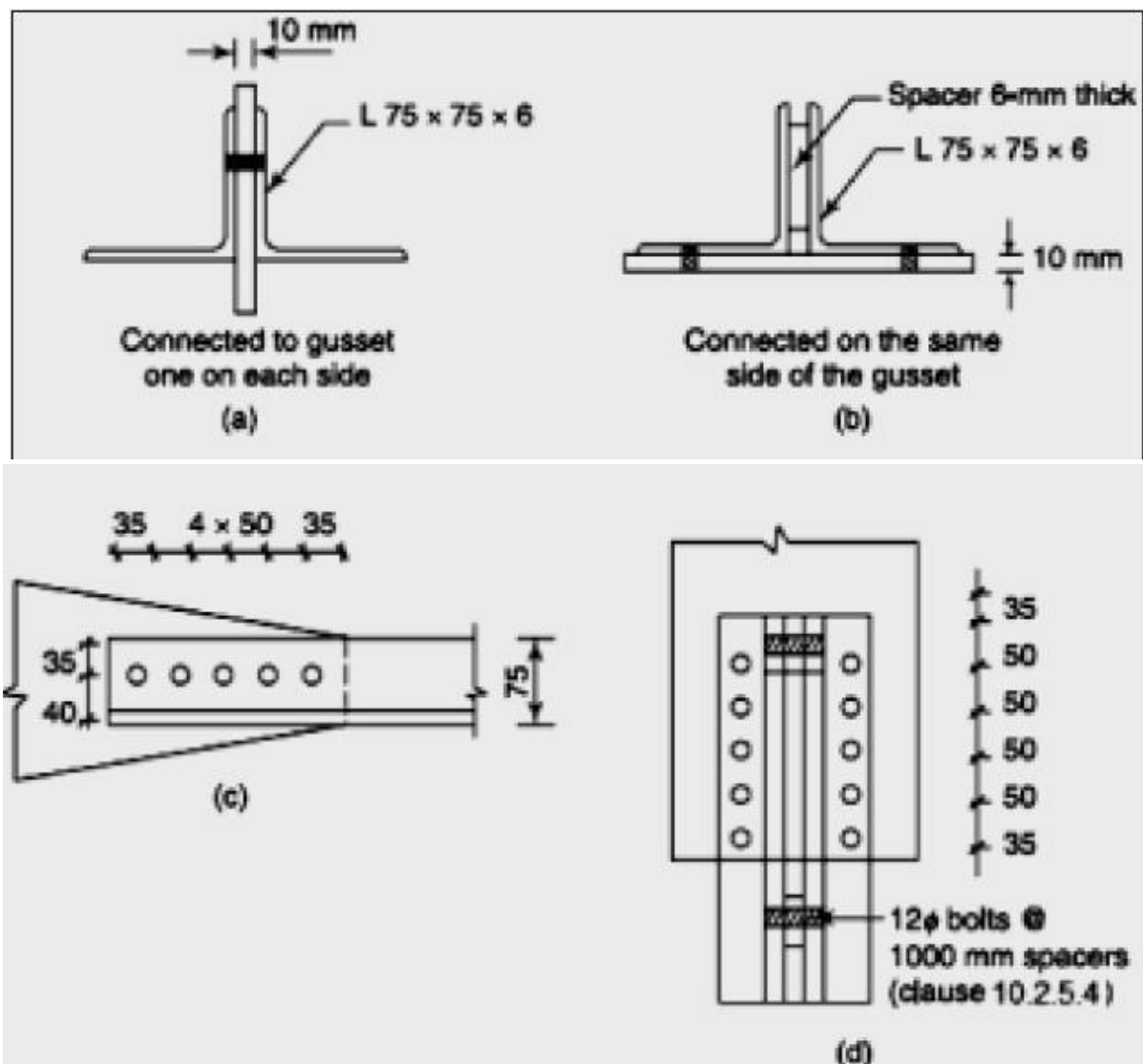
Figure 10.17 Example problem Sample Questions in Steel Structures
