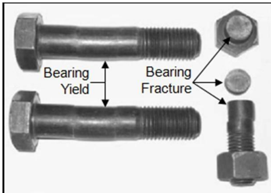
Figure 10.14 Bearing failure of bolts
