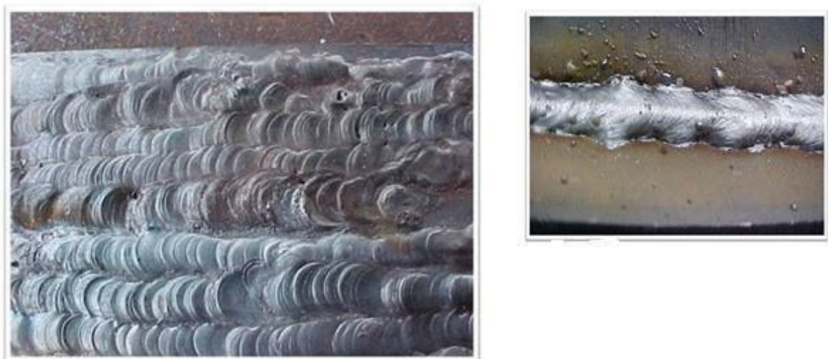
Figure 7.23 unacceptable weld profiles
