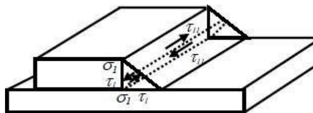
Figure 8.8 Average stress in the weld throat
