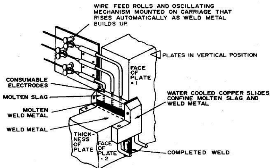
Figure 7.5 Electroslag welding process Stud
