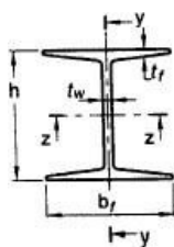
Rolled I-Sections
