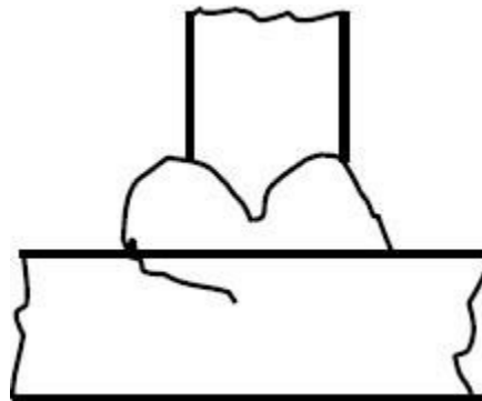
Figure 7.22 Lamellar tear
