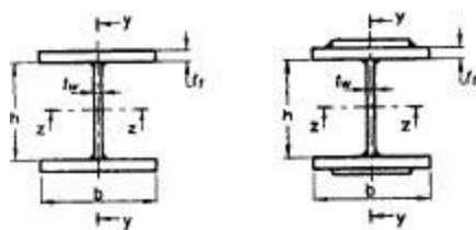
welded I-Section
