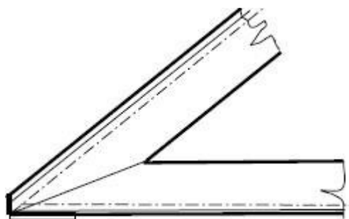
Figure 8.20 Eaves connection Eccentricities
