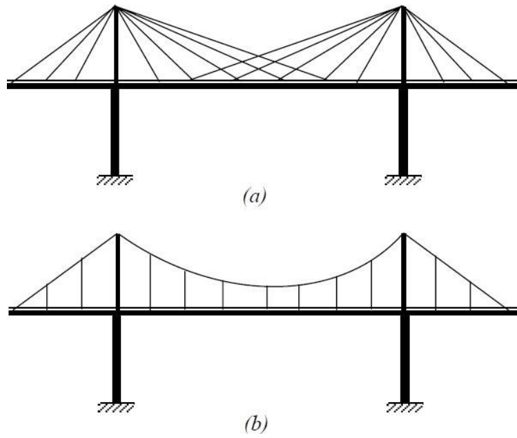
Figure 2.7 Cable-stayed structures
