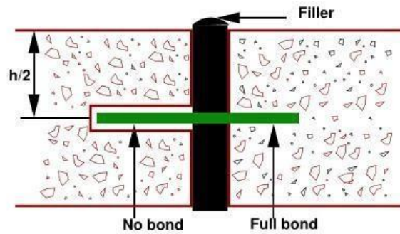
Fig. 35.1 Expansion joint Contraction
