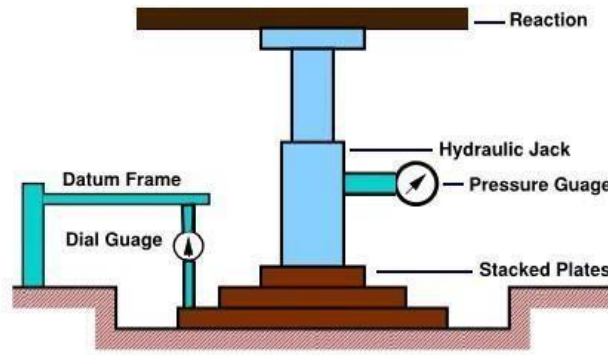
Fig.21.2 Plate load test
