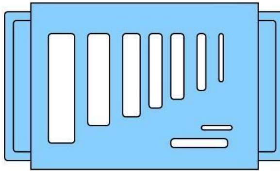
Fig.24.1 Flakiness gauge
