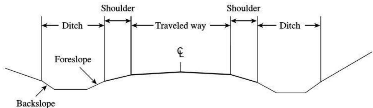
Fig.5.1. Two-lane highway cross section, with ditches.
